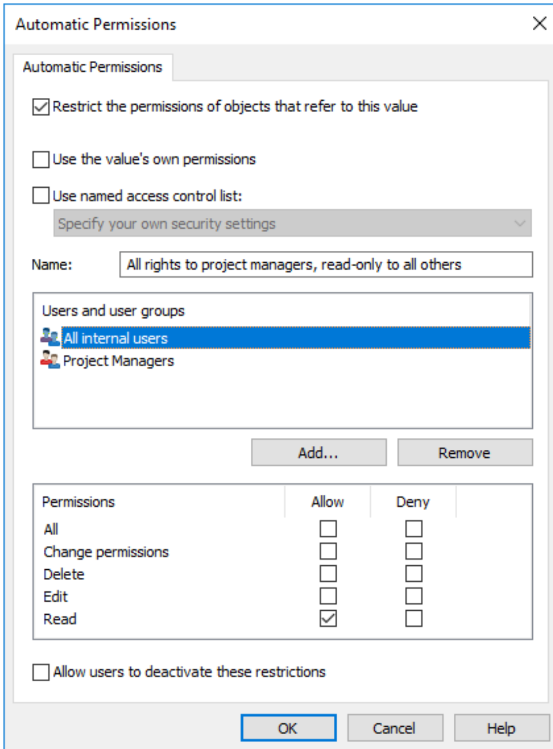
Figure 42: The "Automatic Permissions" dialog for a value list item.
