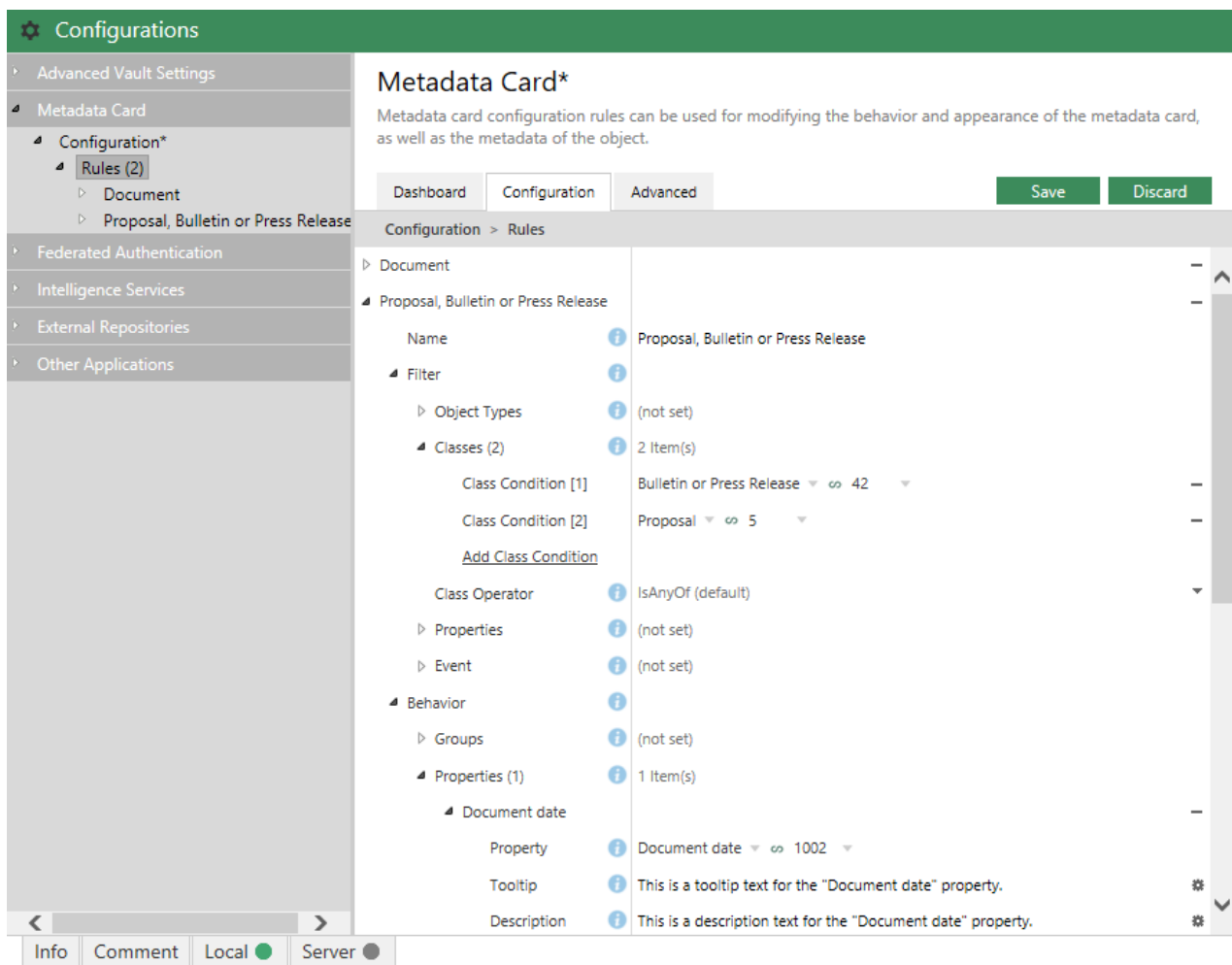
Figure 64: Metadata card configurations in the Configurations editor.
